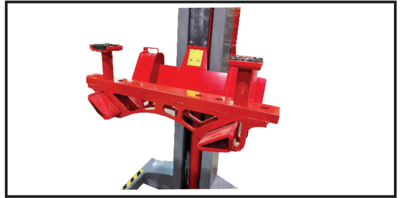
▲ LIGHT TRUCK ADAPTER USED IN PAIRS TO LIFT BY THE FRONT & REAR OF LIGHT TRUCKS #MCOLTA
