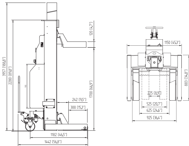
EQUIPMENT FOOTPRINT MCO19B-4-76
