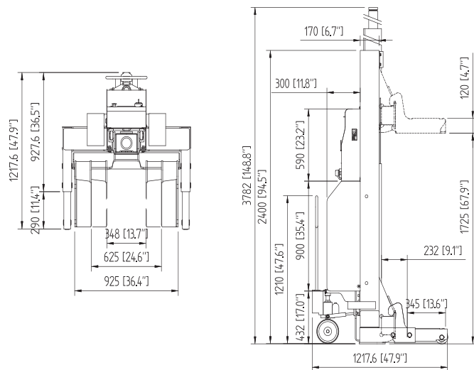
EQUIPMENT FOOTPRINT MCO14.5B-4-58
